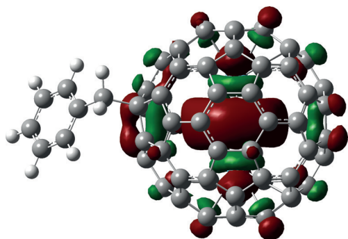
Figure 6. SOMO isoelectronic plot of 2 calculated at the B3LYP/6-31G(d) \approx sdd level.
